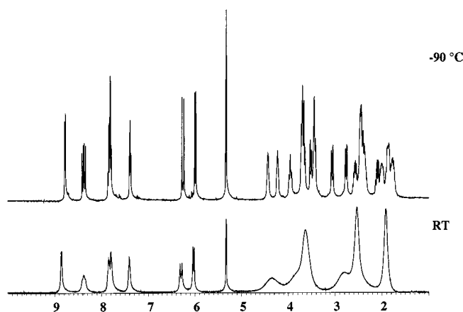
Figure 4. 1 H-NMR spectrum of [Rh(cod)(morpholine)(2-vinylpyridine)][CF 3 SO 3 ] ( 13 ) at room temperature and at –90°C in CD 2 Cl 2
