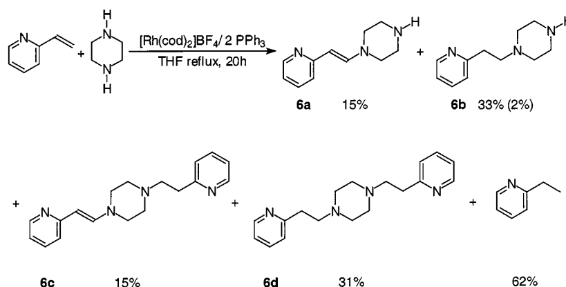
Scheme 3. Reaction of 2-vinylpyridine and piperazine; the yields obtained without catalyst are given in parentheses
