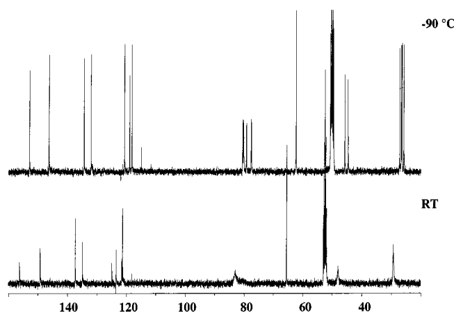
Figure 5. 13 C-NMR spectrum of [Rh(cod)(morpholine)(2-vinylpyridine)][CF 3 SO 3 ] ( 13 ) at room temperature and –90°C in CDCl 3
