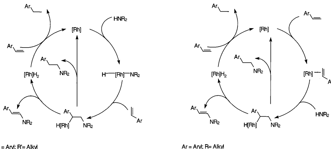
Scheme 4. Catalytic cycles for the amination of aromatic olefins by (a) amine activation and (b) olefin activation
