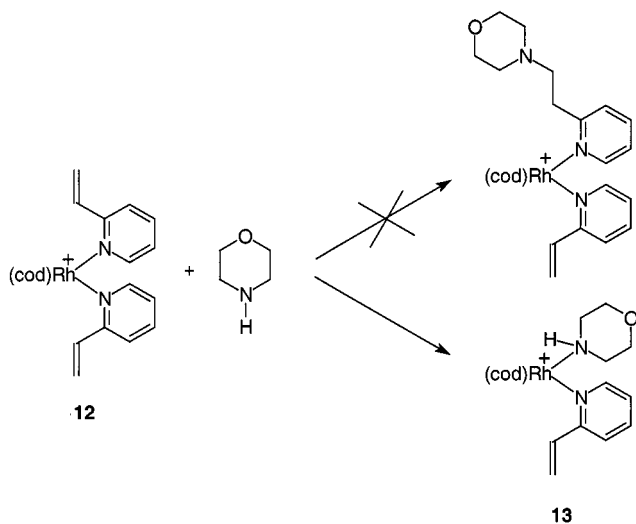
Scheme 6. Reaction of [Rh(cod)(2-vinylpyridine) 2 ][CF 3 SO 3 ] ( 12 ) with morpholine
