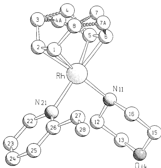
Figure 6. The molecular structure of [\text{Rh}(\text{cod})(\text{morpholine})-(2\text{-vinylpyridine})]^+ \text{CF}_3\text{SO}_3^-
