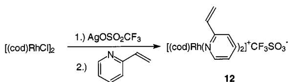
Scheme 5. Synthesis of the cationic complex [\text{Rh}(\text{cod})(2\text{-vinylpyridine})_2]^+\text{CF}_3\text{SO}_3^- ( 12 )
