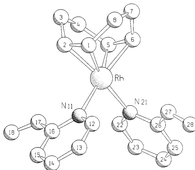
Figure 3. The molecular structure of [\text{Rh}(\text{cod})(2\text{-vinylpyridine})_2]^+
