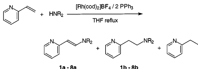
Scheme 2. Rhodium-catalyzed amination of 2-vinylpyridine
